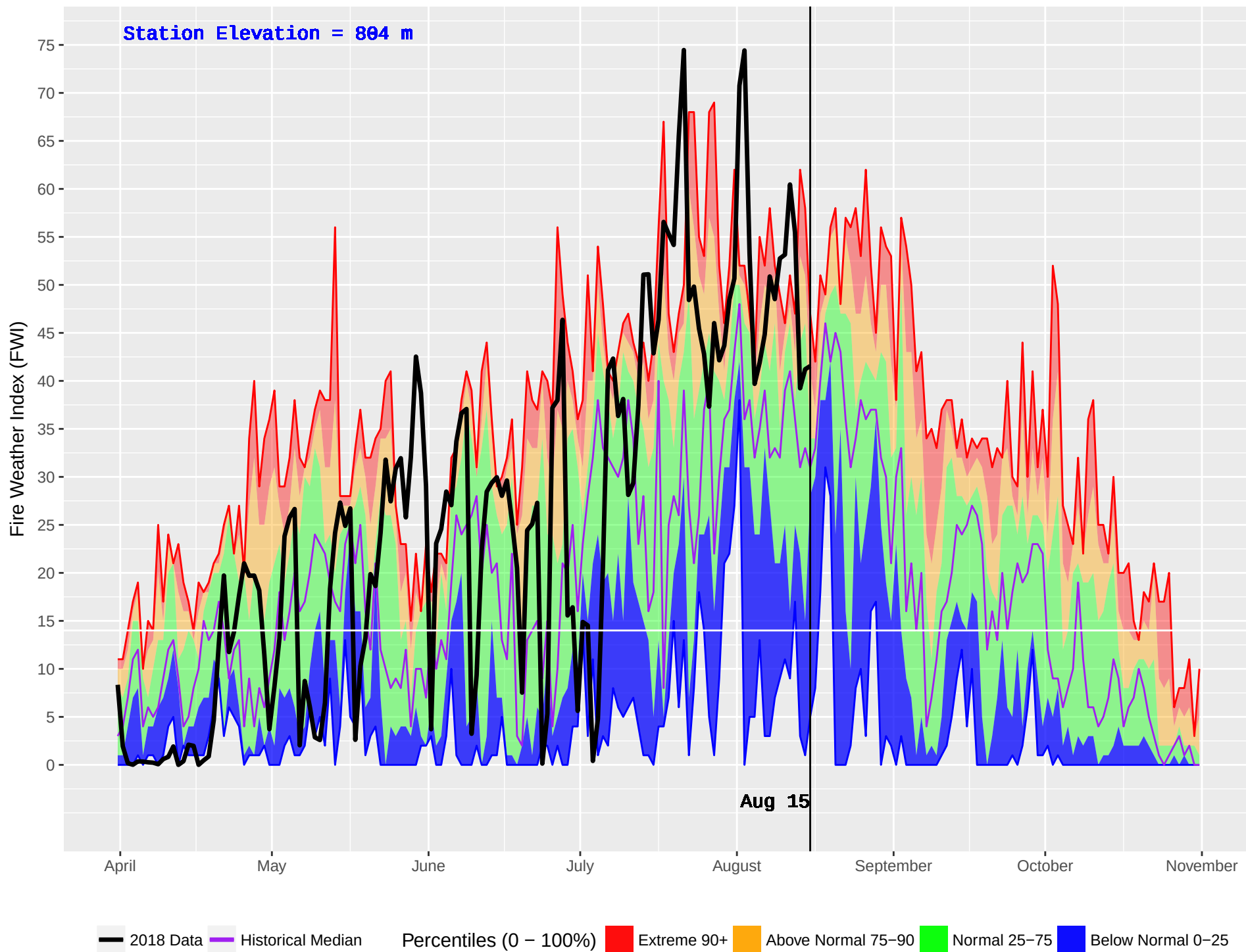
KOOCANUSA (1075) : Historical (2010–2016) and Current (2018) Daily Fire Weather Index (FWI)
